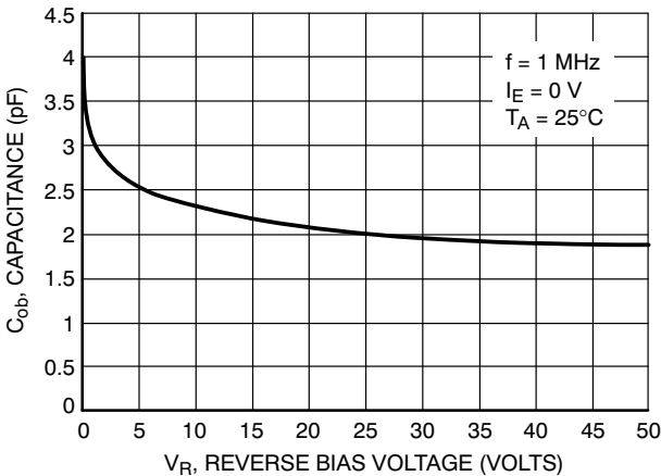
Figure 34. Output Capacitance
