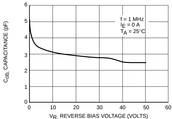
Figure 24. Output Capacitance
